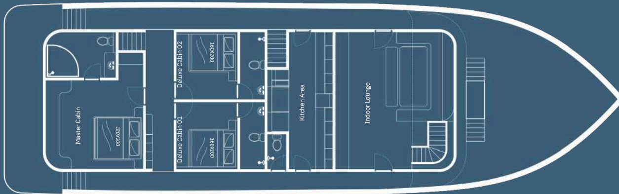
Main Deck
